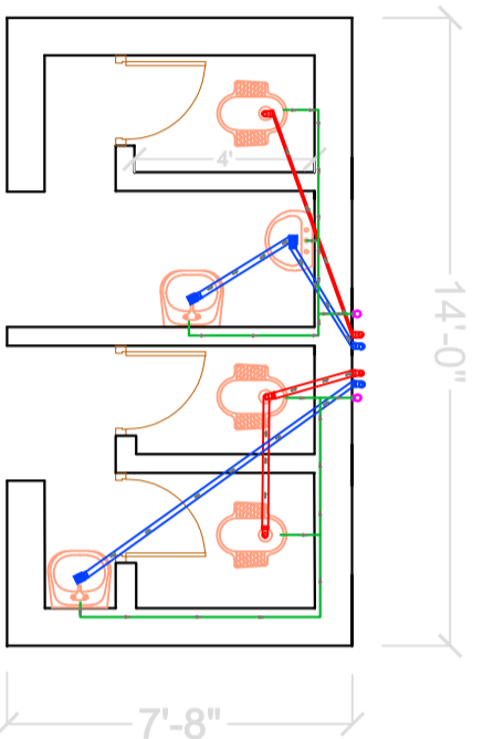
PLUMBING DRAWING
